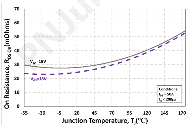
Figure 5. On-Resistance vs. Temperature
