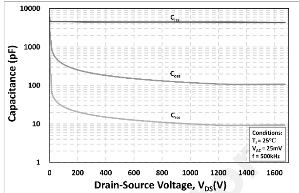
Figure 26. Capacitances vs. Drain-Source Voltage (0 - 1700V)
