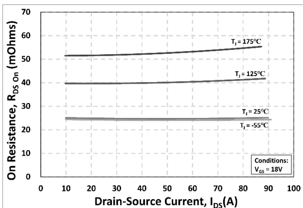
Figure 6. On-Resistance vs. Drain Current Various Temperatures
