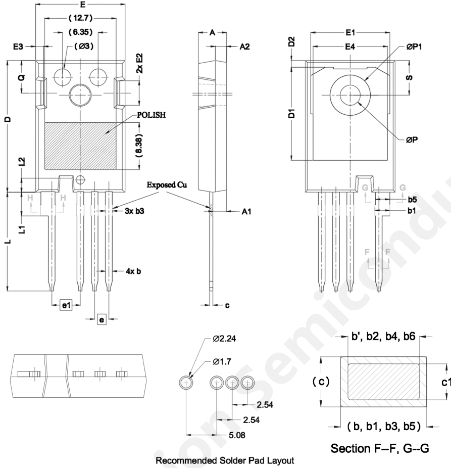
Drawing and Dimensions
