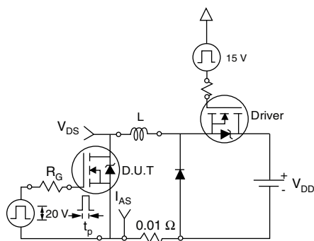
Fig. 19 - Unclamped Inductive Test Circuit
