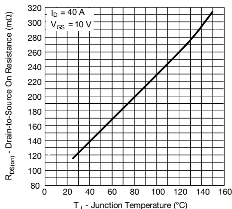
Fig. 6 - Normalized On-Resistance vs. Temperature
