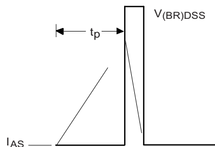
Fig. 20 - Unclamped Inductive Waveforms
