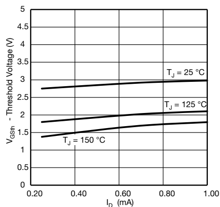
Fig. 10 - Typical MOSFET Threshold Voltage
