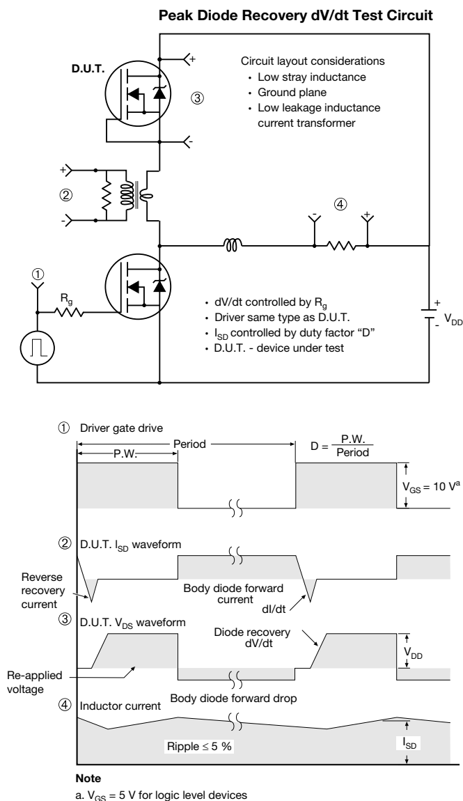
Fig. 20 - For N-Channel
