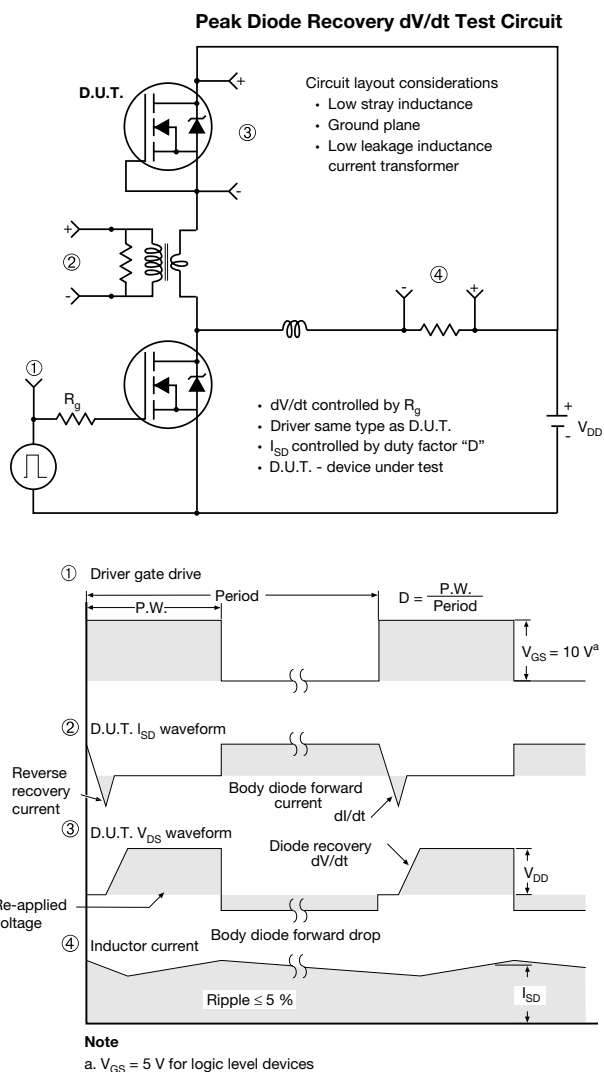
Fig. 14 - For N-Channel
