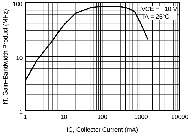
Figure 10. f_T - I_C
