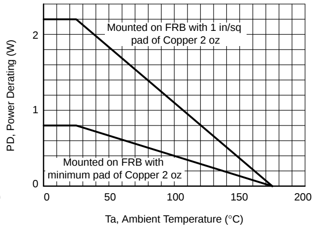
Figure 13. Power Derating
