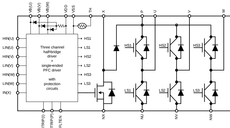
Figure 1. Function Diagram
