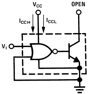
FIGURE 11. I CCH , I CCL for OR, NOR Circuits
