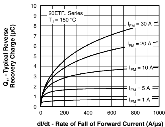
Fig. 13 - Recovery Current Characteristics, T_J = 150\text{ }^{\circ}\text{C}
