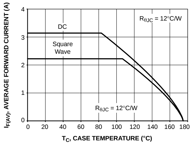
Figure 6. Current Derating
