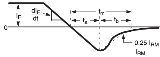
Figure 14. t_{rr} Waveforms and Definitions
