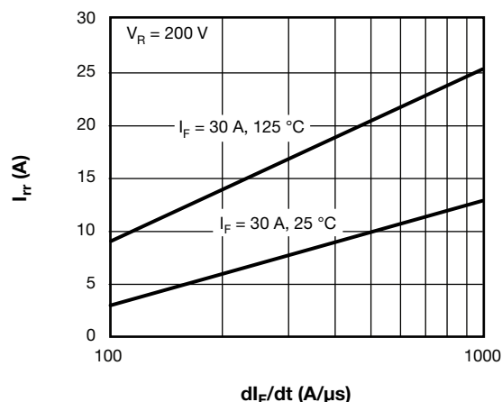
Fig. 9 - Typical Stored Current vs. dl_F/dt
