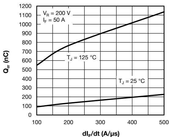
Fig. 8 - Reverse Recovery Charge vs. dI_F/dt
