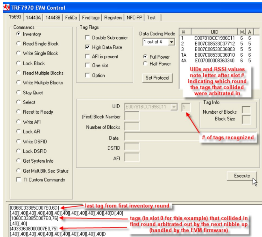
Figure 6. Sixteen Slot Inventory Command (Five Tags in Field, Collision in Slot 0)
