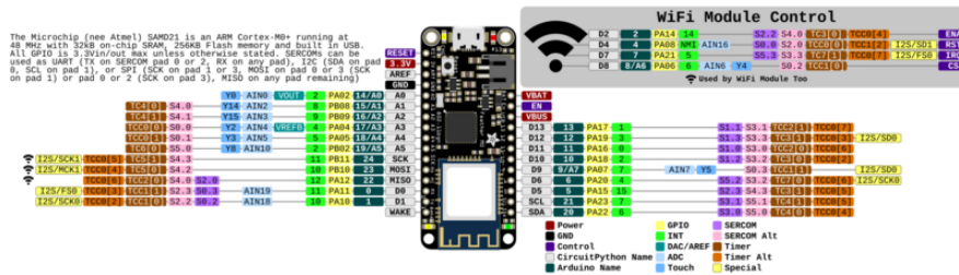
Adafruit Feather M0 WINC1500 https://www.adafruit.com/products/3010
