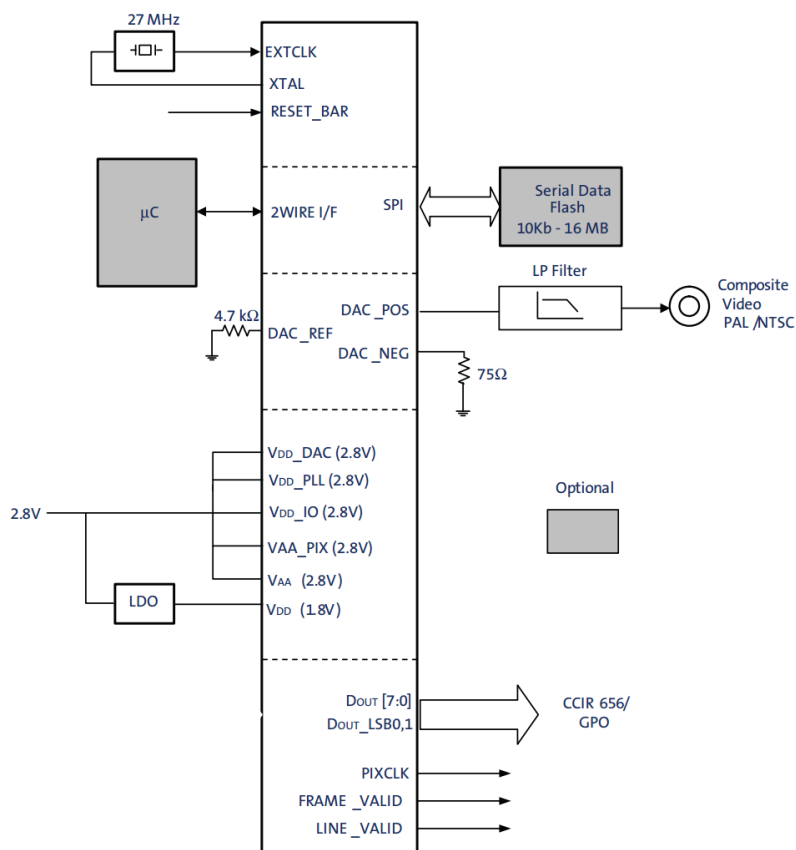
Figure 2. Block Diagram of MT9V136C12STCH-GEVB
