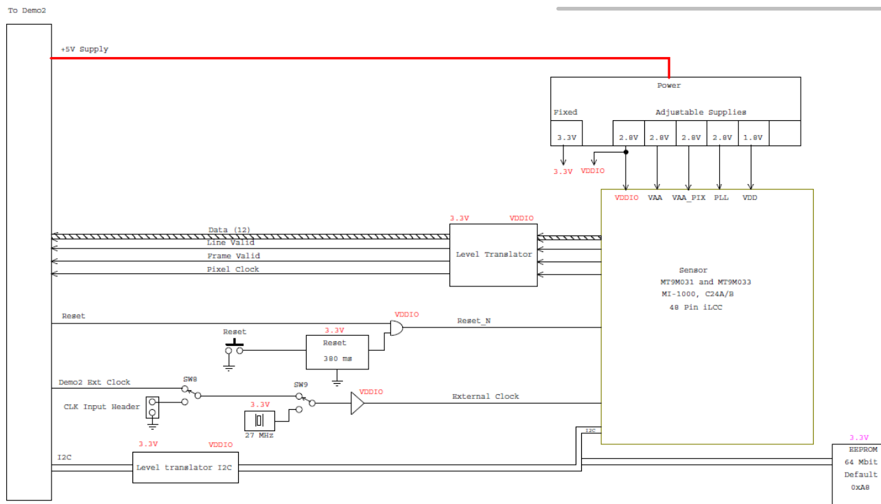
Figure 2. Block Diagram of MT9M031I12STMZH-GEVB
