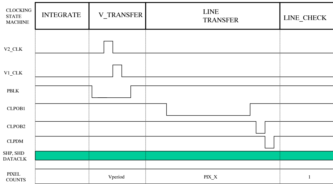
Figure 11. AD9845A Timing
