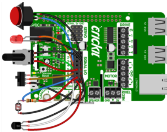
fritzing
