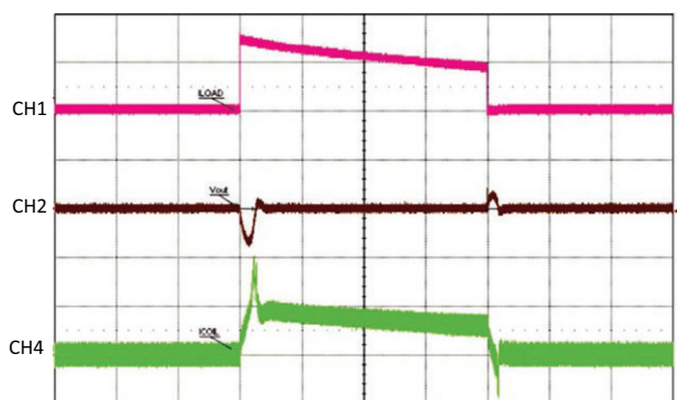
Fig. 12 - Load Step 0 A to 5 A to 0 A CH1 = I_{load} , CH2 = V_{OUT} , 500 mV/div, CH4 = I_{coil} , 5 A/div, Time = 100 \mu\text{s/div}
