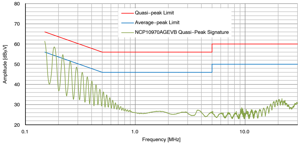
Figure 9. Quasi-Peak EMI Measurement NCP10970AGEVB, V_{IN} = 230 V_{rms} , I_{OUT} = 44 mA , I_{LDOUT} = 94 mA
