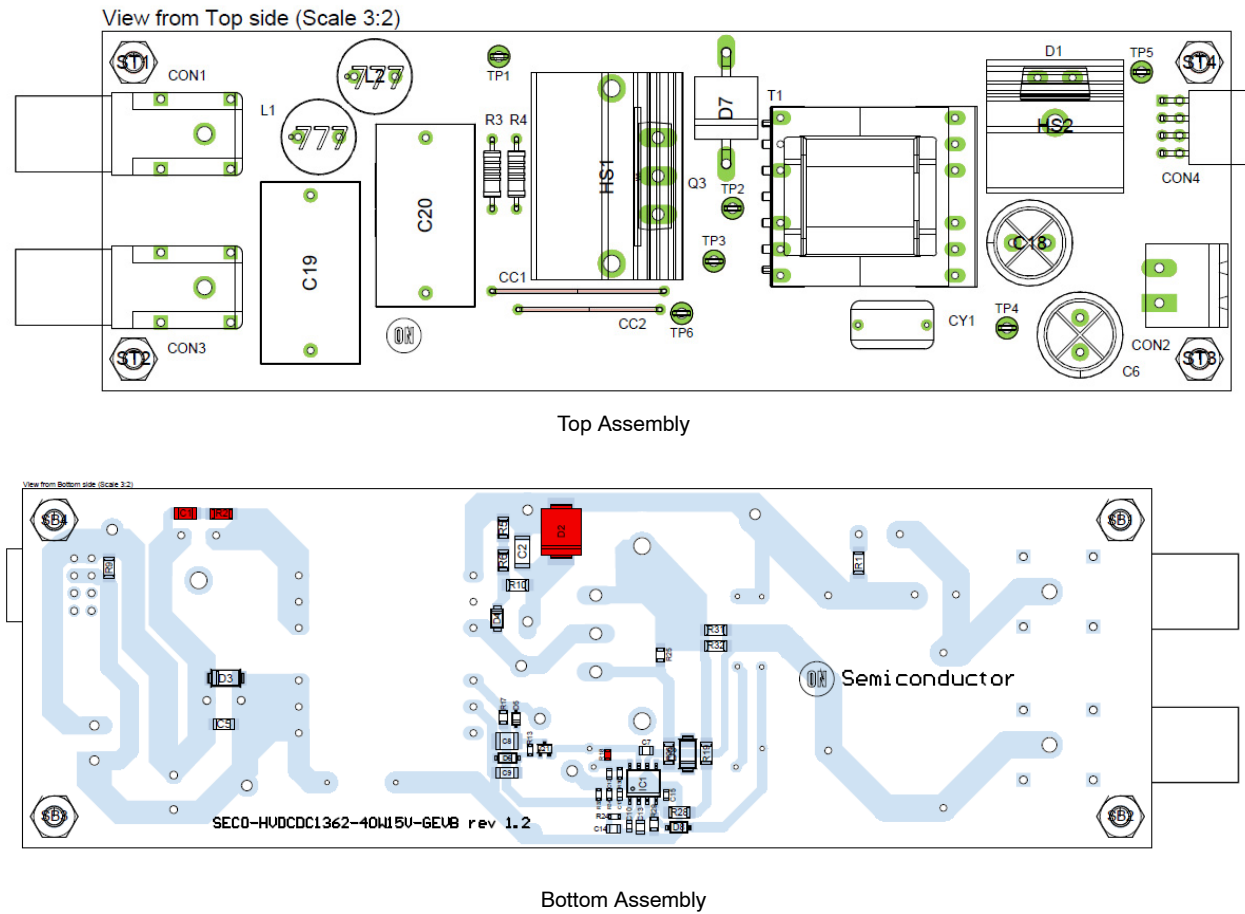
Figure 22. Layout
