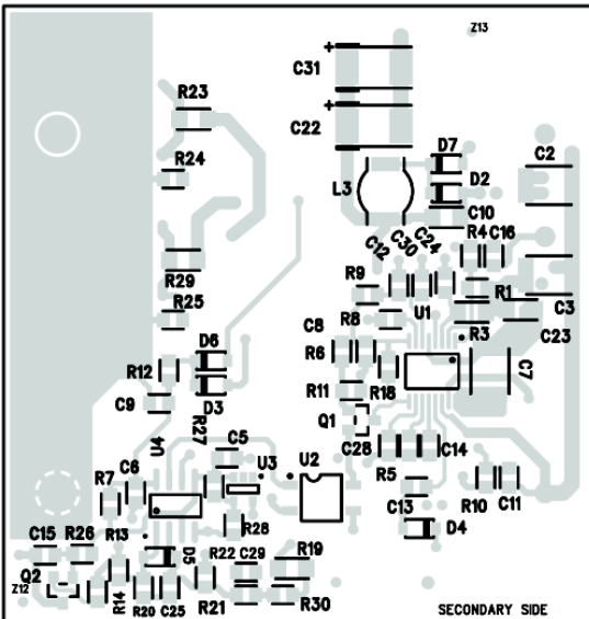
Figure 25. Layer 4 (Bottom)
