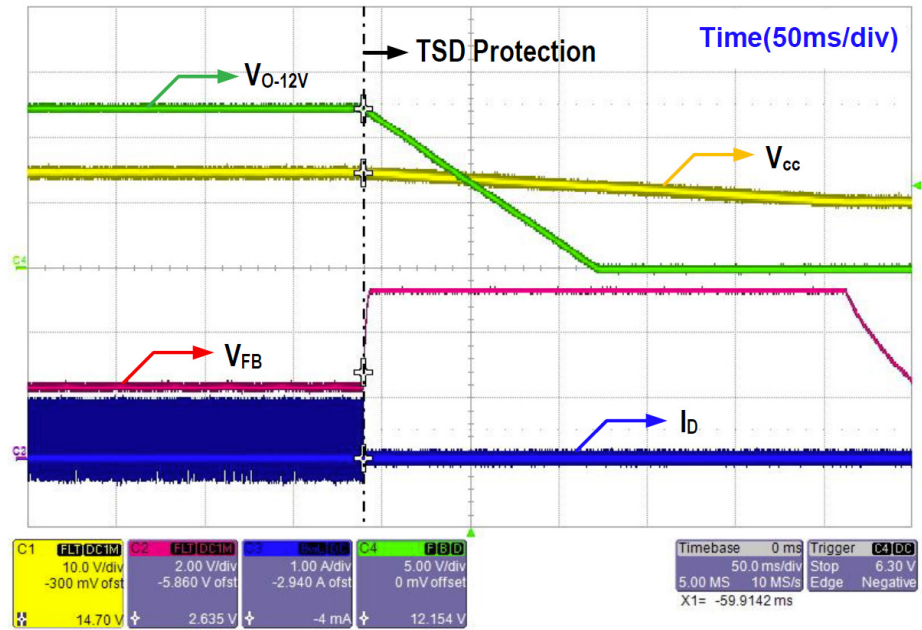
Figure 40. TSD @ 115 V_{AC} /60 Hz, Full Load
