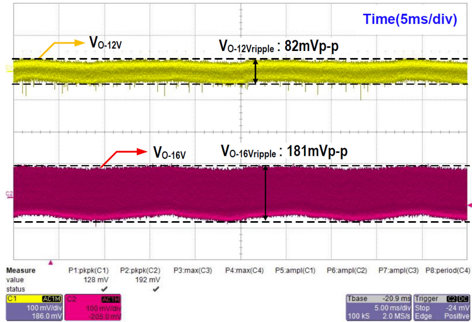
Figure 19. Output Ripple Voltage @230 V_{AC} /60 Hz, Full Load
