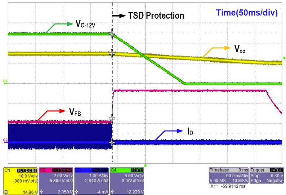
Figure 41. TSD @ 230 V_{AC} /60 Hz, Full Load
