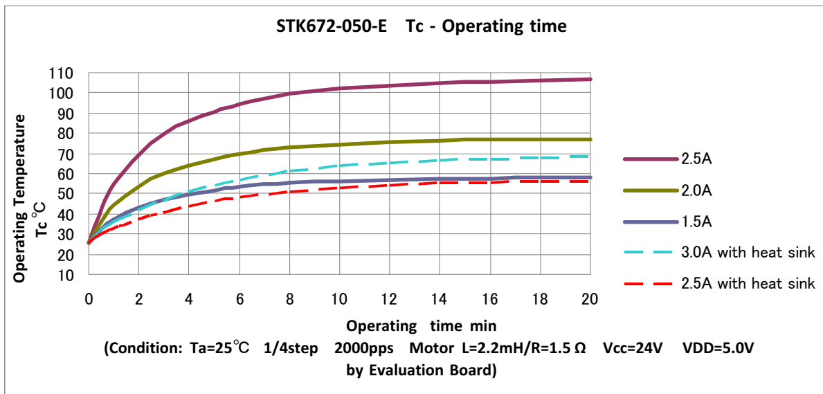
Figure 7. Operating Temperature
