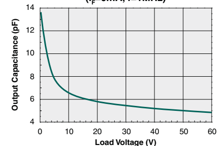
Output Capacitance vs. Load Voltage ( I_F=0\text{mA} , f=1\text{MHz} )
