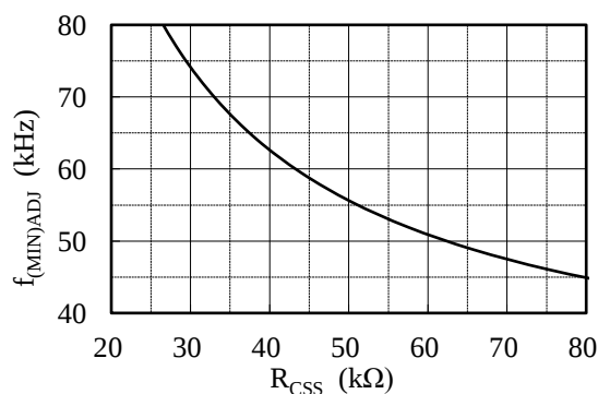
Figure 8-18. R5 ( R_{CSS} ) vs. f_{(MIN)ADJ}
