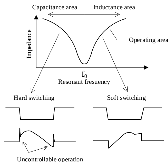
Figure 8-30. Operating Area of Resonant Power Supply
