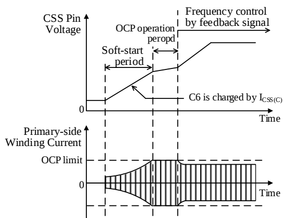
Figure 8-17. Soft-start Operation
