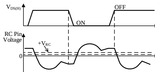
Figure 8-31. RC Pin Voltage in Inductance Area
