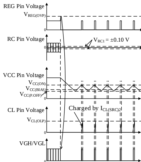
Figure 8-39. REG_OVP Waveform
