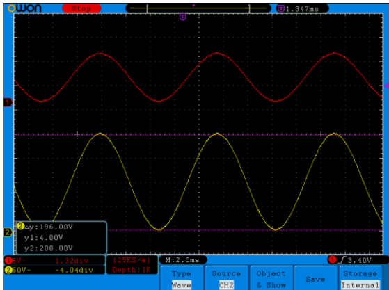
Figure 7. f=100Hz
