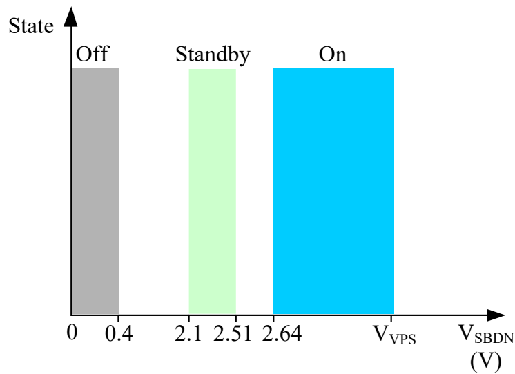
Figure 3. V_{SBDN} vs. Amplifier States
