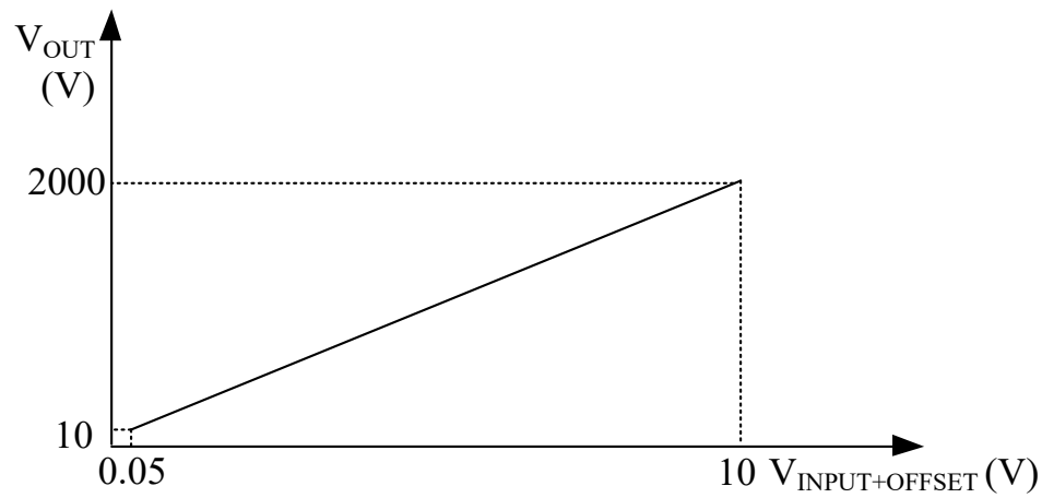
Figure 2. V_{INPUT+OFFSET} vs. V_{OUT}
