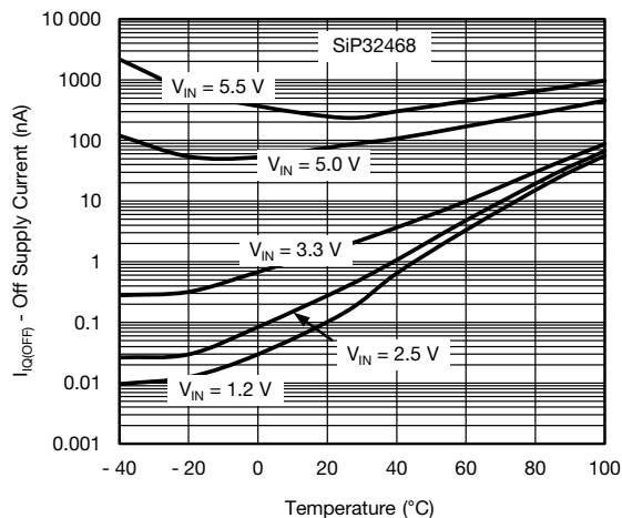
Fig. 6 - Off Supply Current vs. Temperature
