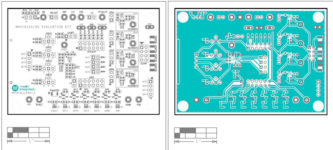
Figure 3. MAX16165/MAX16166 EV Kit PCB Layout—Top Silkscreen MAX16165/MAX16166 EV Kit PCB Layout—Top
