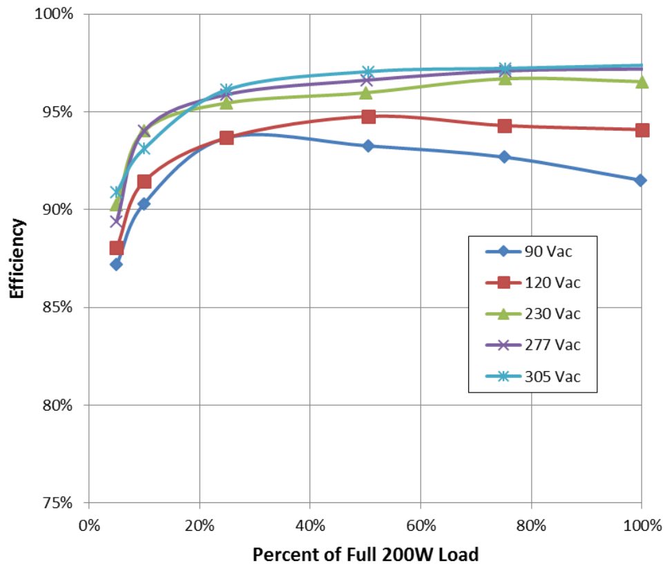
Figure 8. Efficiency
