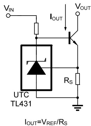
Constant-current Sink
