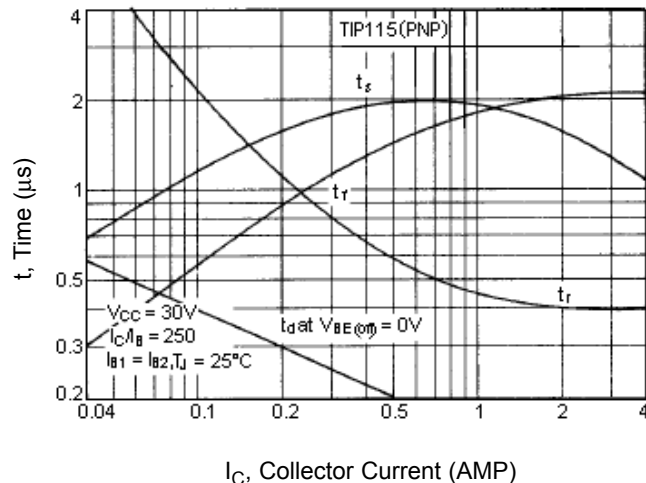
Figure - 3 Switching Time
