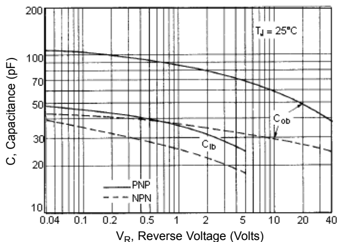
Figure - 4 Capacitances
