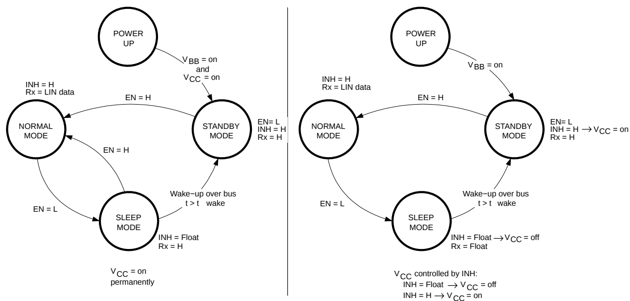
Figure 3. State Diagrams
