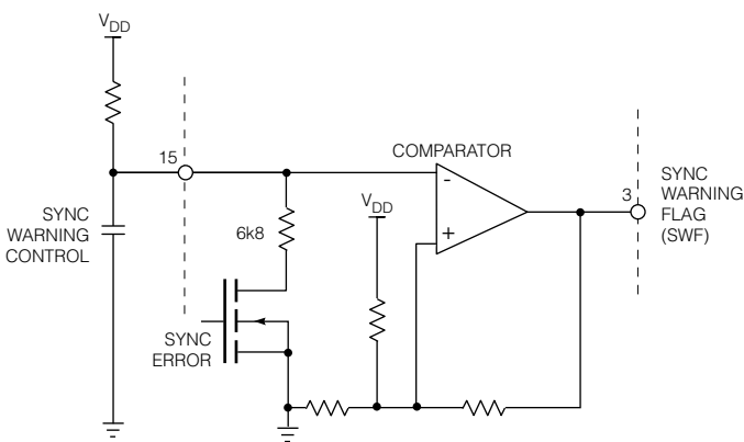
Fig. 10 Sync Warning Flag Circuit
