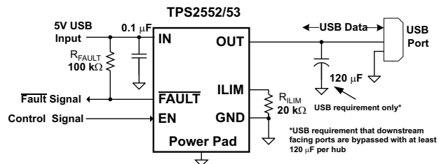
Figure 1. Typical Application as USB Power Switch
