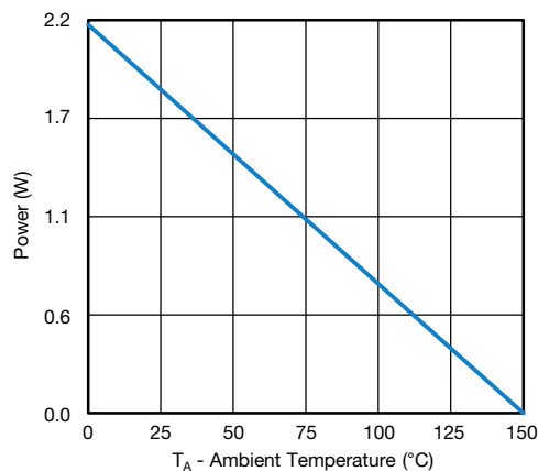
Power, Junction-to-Ambient
