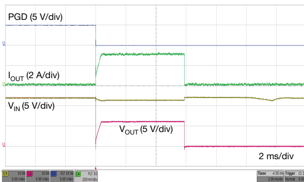
Fig. 31 - Output Short With a 2\text{ }\Omega Load V_{IN} = 12\text{ V} , R_L = 2\text{ }\Omega , C_{SS} = 133\text{ nF} , R_{LIM} = 1.74\text{ k}\Omega
