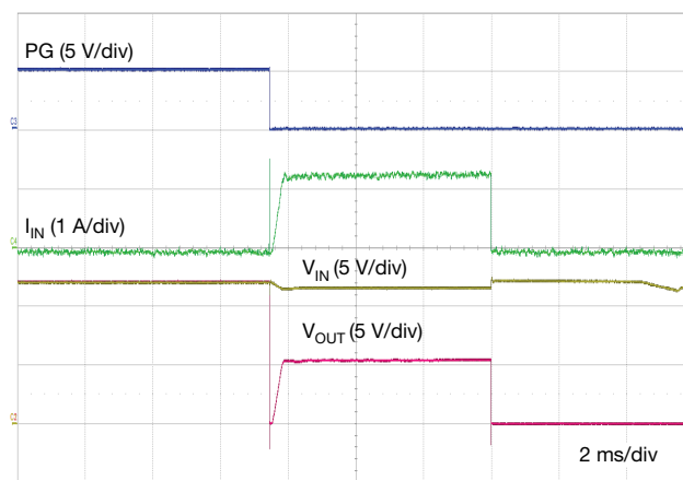
Fig. 29 - V OUT Short With a 2 Ω Load V IN = 12 V, R L = 2 Ω, C L = 0 μF, C SS = 133 nF, R LIM = 2.49 kΩ
