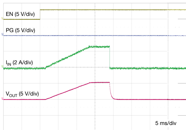
Fig. 28 - Turn On by EN Into OCP Load V IN = 12 V, R L = 2 Ω, C L = 47 μF x 3, C SS = 133 μF, R LIM = 2.49 kΩ
