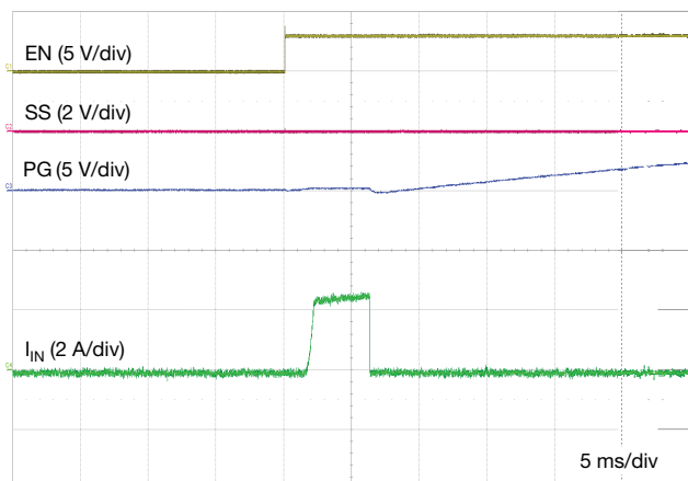
Fig. 26 - Turn On Into Output Short V IN = 12 V, C SS = 133 nF, R LIM = 2.49 kΩ
