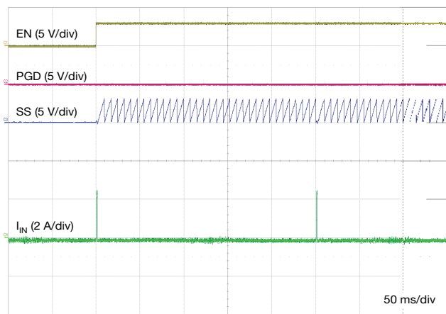
Fig. 27 - Turn On Into Output Short, Auto-Retry V IN = 12 V, C SS = 133 nF, R LIM = 2.49 kΩ
