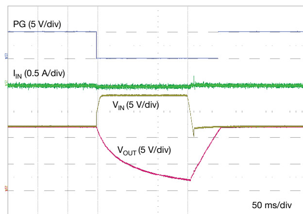
Fig. 31 - Over Voltage Protection R L = 1 kΩ, C L = 100 μF, C SS = 133 nF, R LIM = 2.49 kΩ, OVP Set to 18 V
