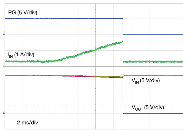
Fig. 30 - Output Current Protection Increase Load Current Slowly V IN = 12 V, R L = 2 Ω, C L = 47 nF, C SS = 133 nF, R LIM = 2.49 kΩ
