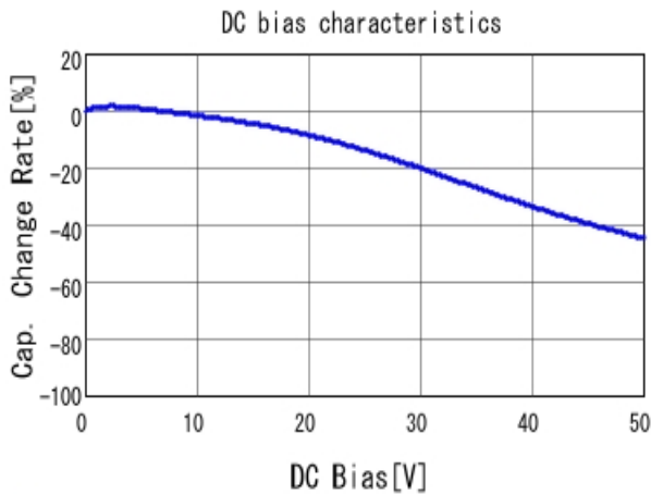
■ GRM155R11H472KA01 C-DC bias capchange, 20.0degC, AC1.
