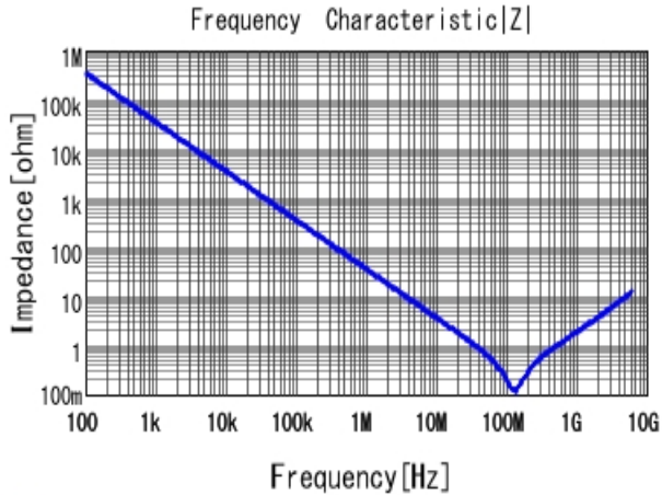
■ GRM155R11H472KA01 |Z| DC0V, 20degC
