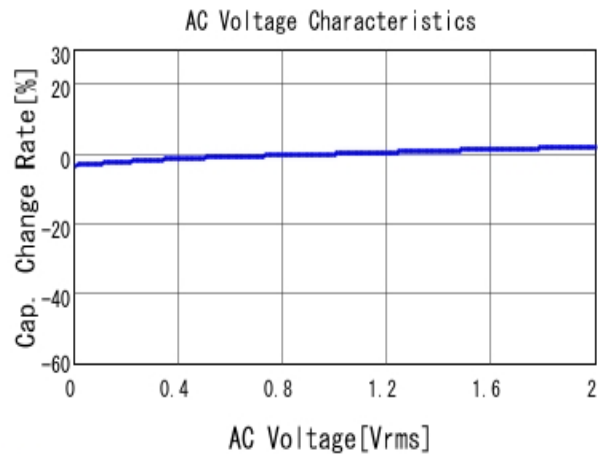
■ GRM155R11H472KA01 C-AC Voltage capchange, DC0V, 20.0d
