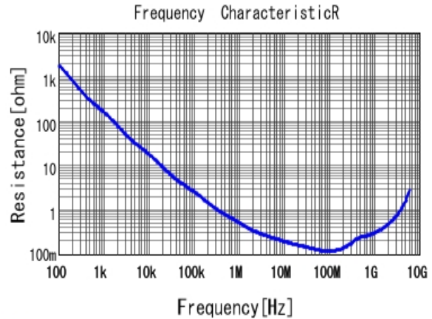
■ GRM155R11H472KA01 R DC0V, 20degC
