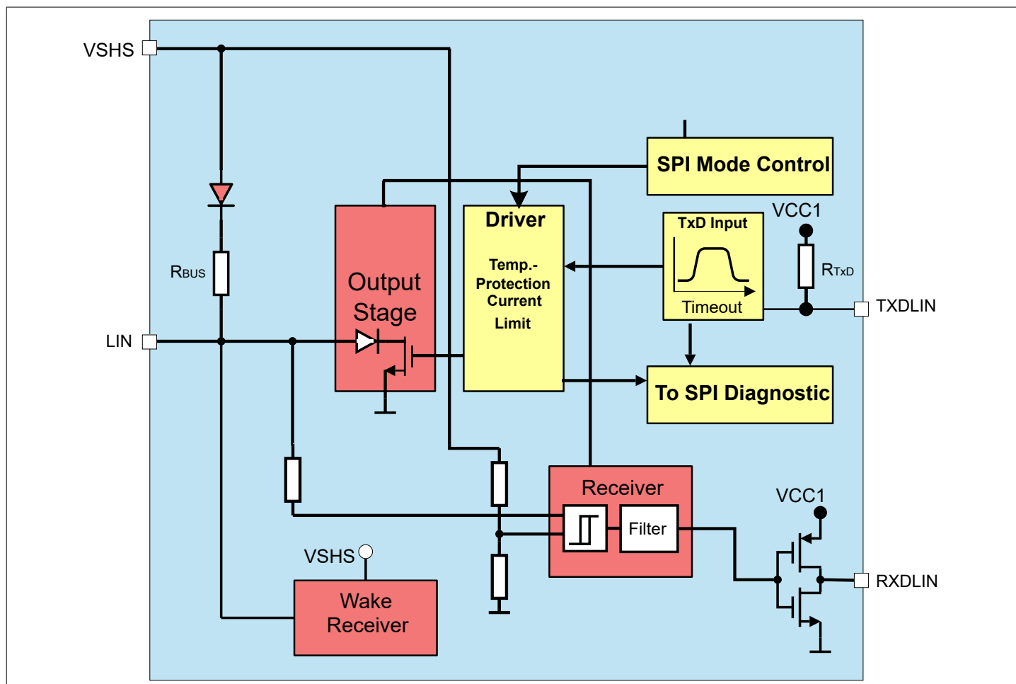
Figure 32 Block Diagram
