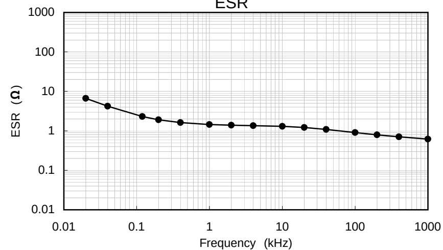
ESR
