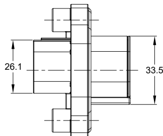
INTERNAL SEALING SURFACE FINISH TO BE \frac{3}{32} OR BETTER
