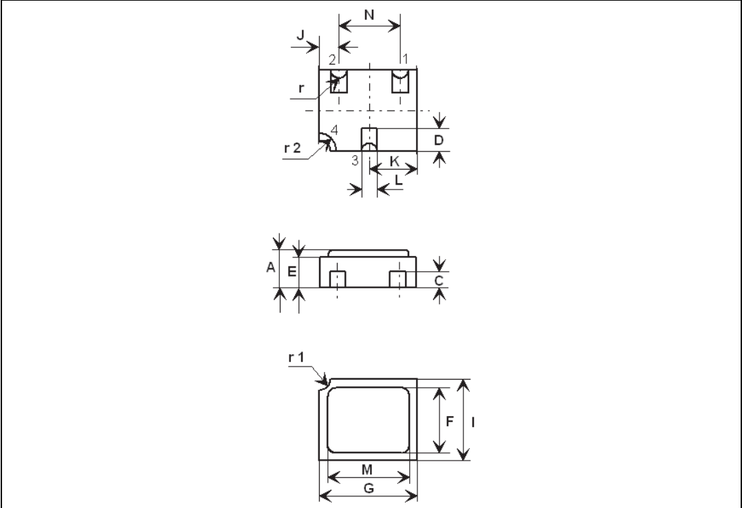
Figure 9. LCC-3UB drawings
