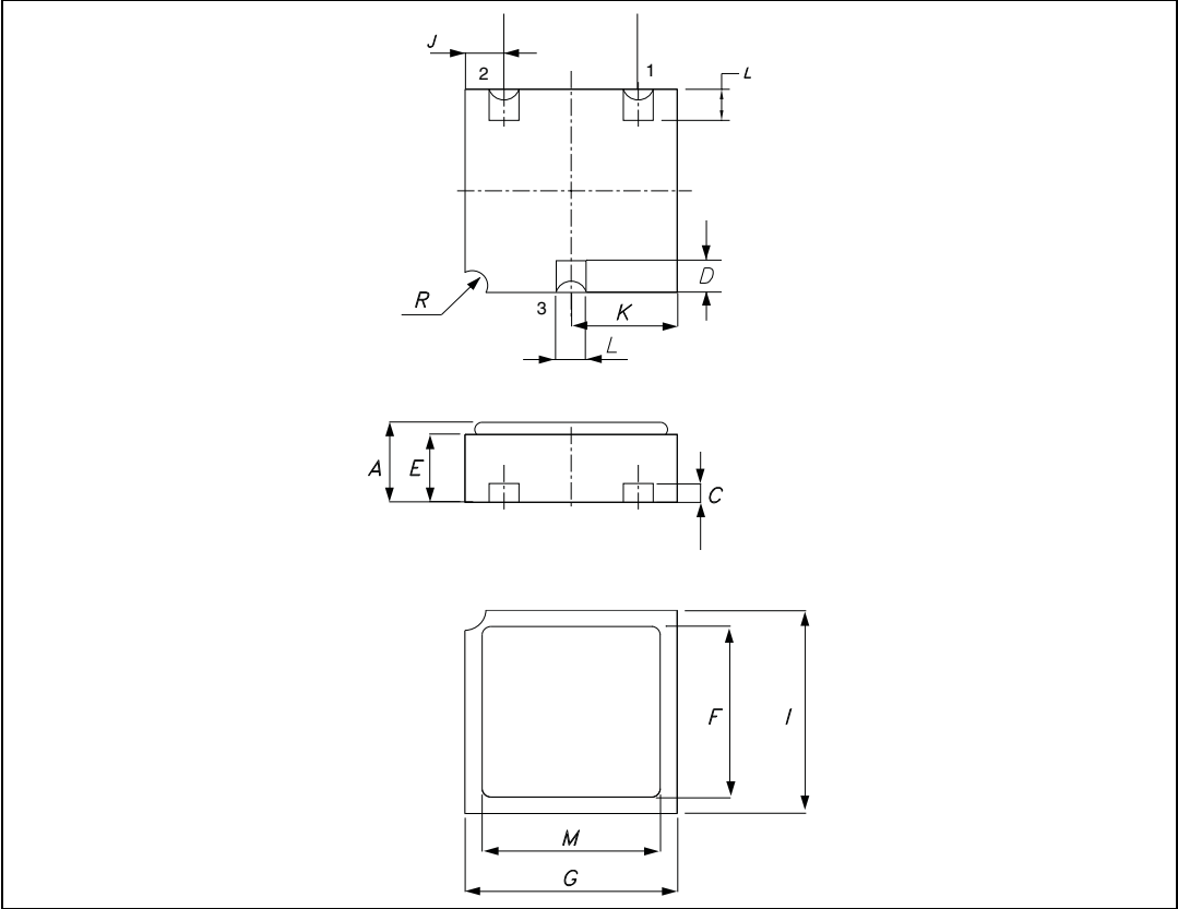
Figure 10. LCC-3 drawings
