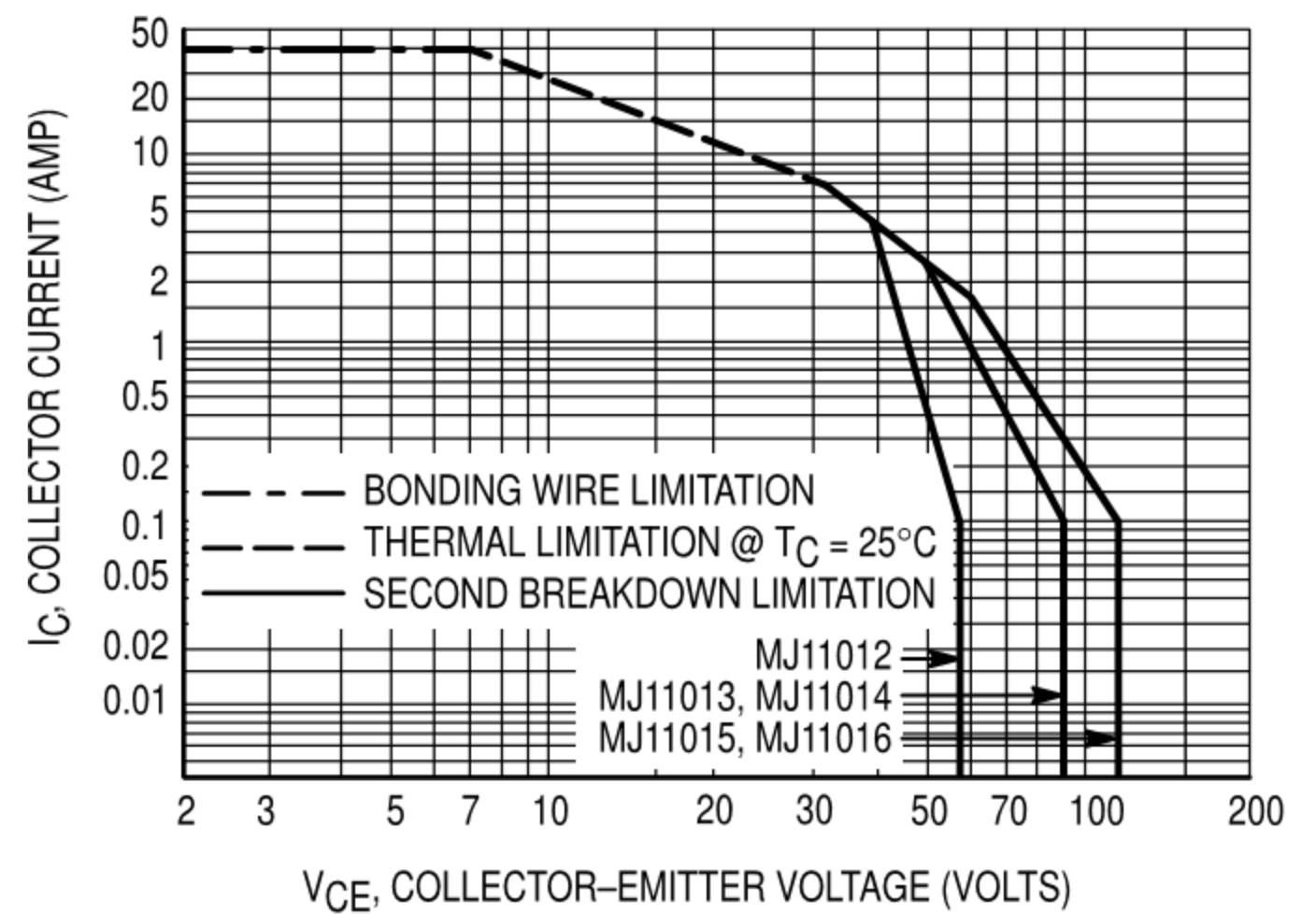
Figure 5. Active Region DC Safe Operating Area
