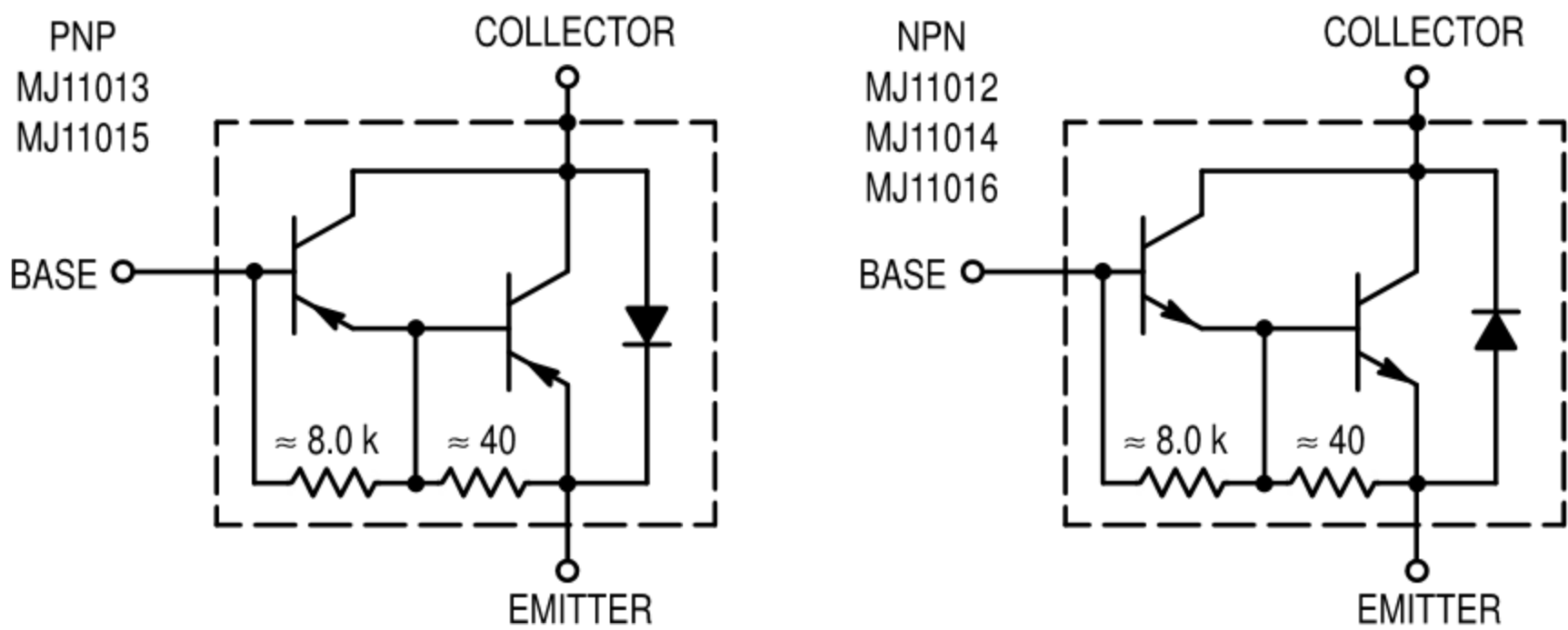
Figure 1. Darlington Circuit Schematic
