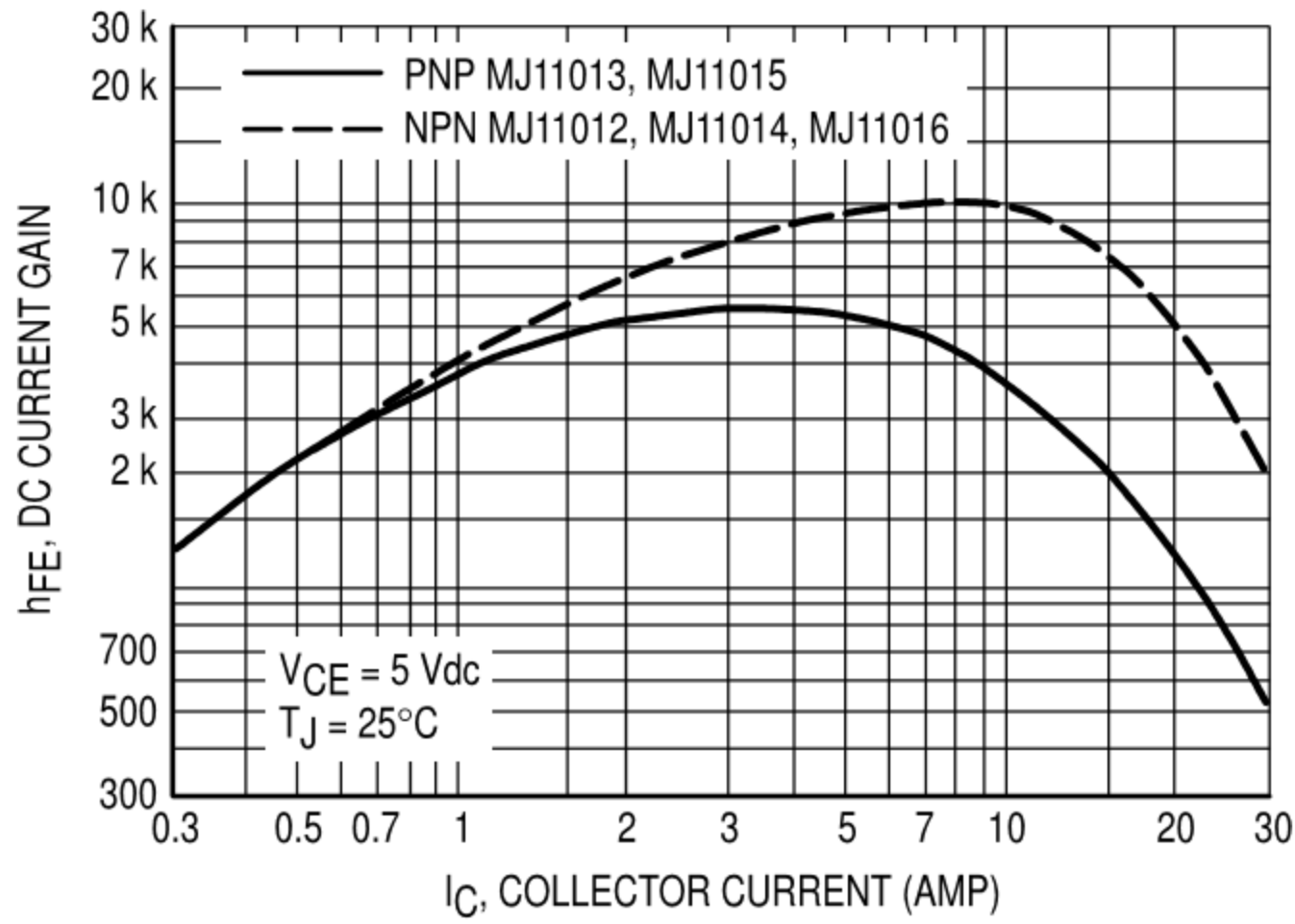
Figure 2. DC Current Gain (1)
