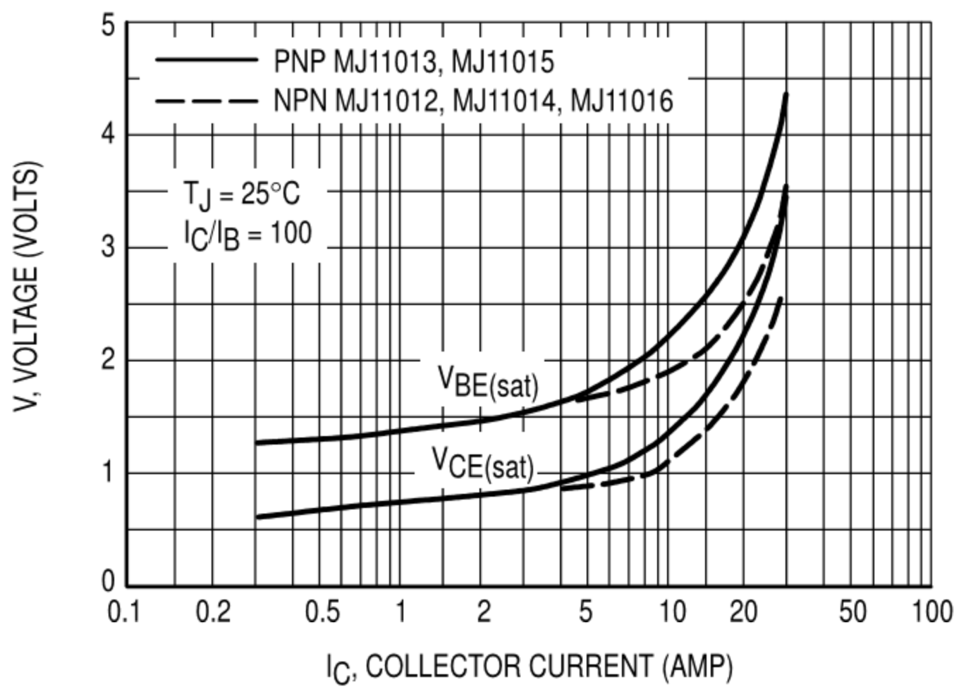
Figure 4. "On" Voltages (1)
