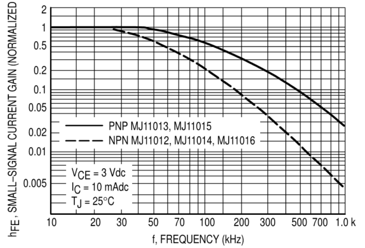
Figure 3. Small-Signal Current Gain
