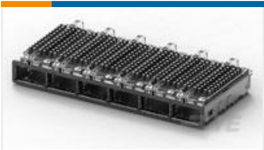
TE Part #2170023-2 1x6 QSFP Kit, Single Sqr LP, SAN Htsnk
