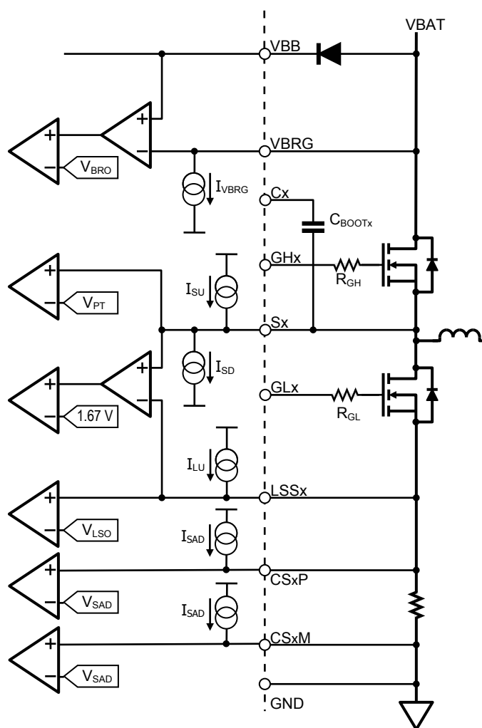
Figure 9: Bridge Terminal Connection Verification
