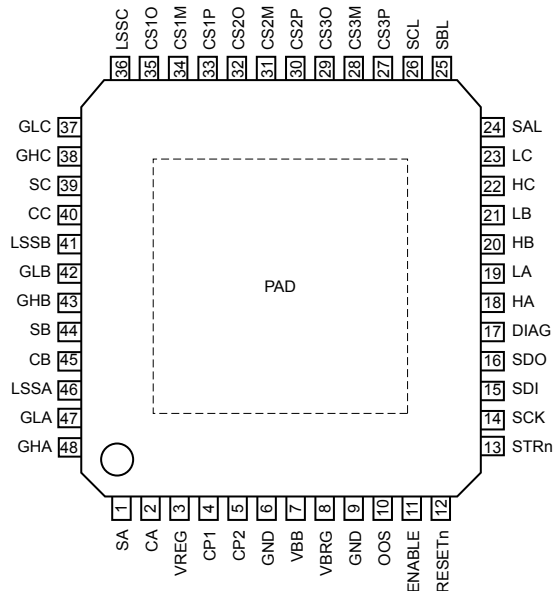
LQFP-48 (JP) Package Pinout Diagram
