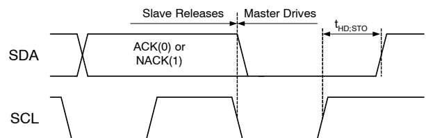
Figure 20. STOP Bit
