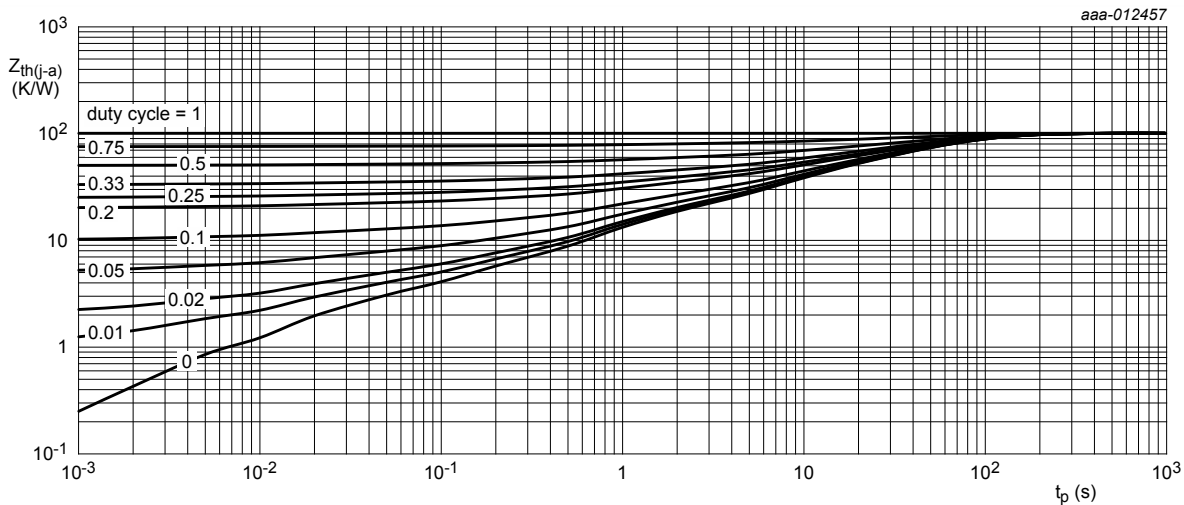
FR4 PCB, mounting pad for cathode 1\text{ cm}^2 Fig. 2. Transient thermal impedance from junction to ambient as a function of pulse duration; typical values
