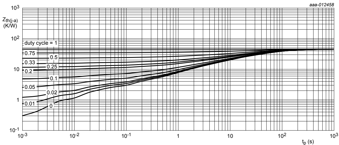
Ceramic PCB, \text{Al}_2\text{O}_3 , standard footprint Fig. 3. Transient thermal impedance from junction to ambient as a function of pulse duration; typical values
