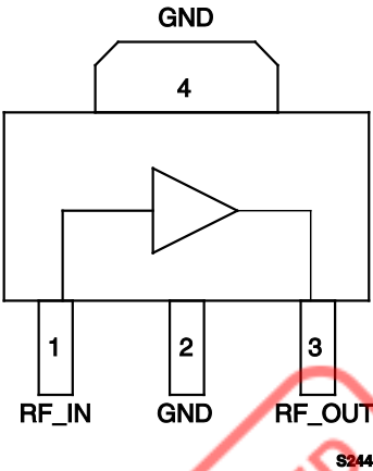
Figure 2. SKY65081-70LF Pinout (Top View)
