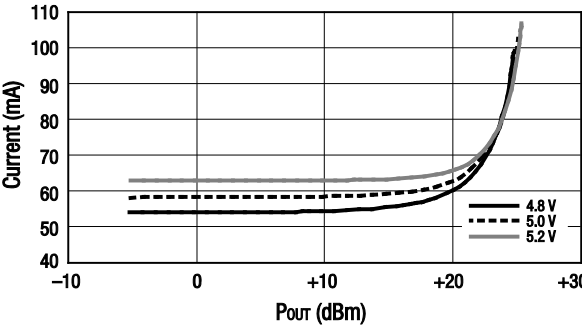
Figure 12. Current vs Output Power Over Voltage
