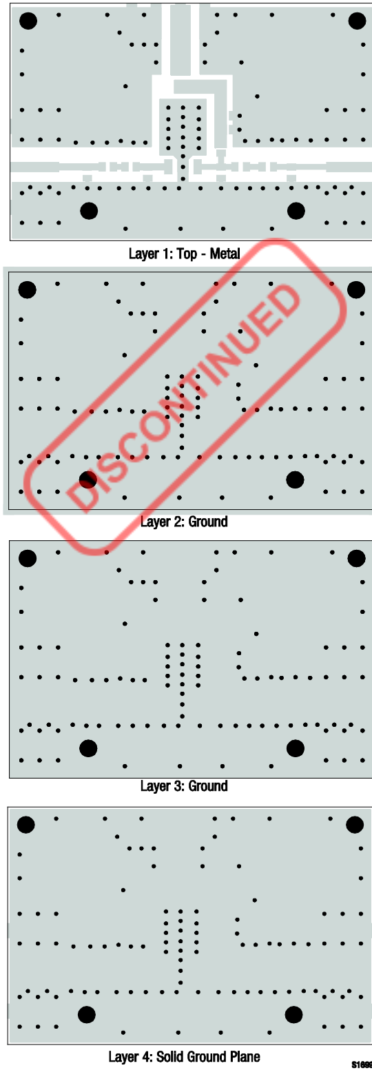
Figure 14. Evaluation Board Layer Detail
