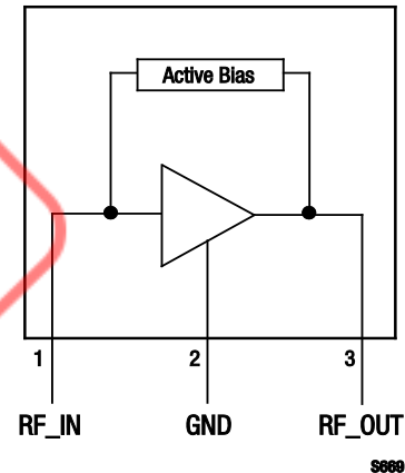
Figure 1. SKY65081-70LF Functional Block Diagram
