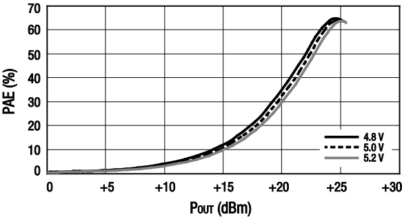
Figure 11. PAE vs Output Power Over Voltage
