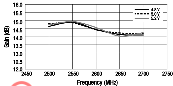
Figure 4. Gain vs Frequency Over Voltage
