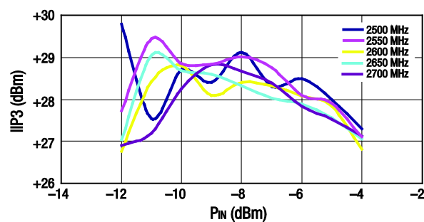
Figure 8. IIP3 vs Input Power Over Frequency
